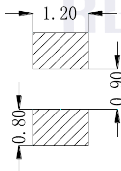
Fig.1-5 Soldering Patterns 推荐焊盘
