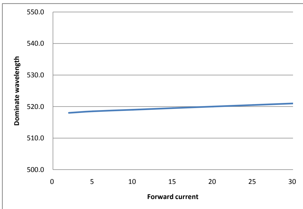
Fig. 1-13 Forward current vs. Dominate wavelength正向电流与主波长特性曲线 (Ts=25°C)
