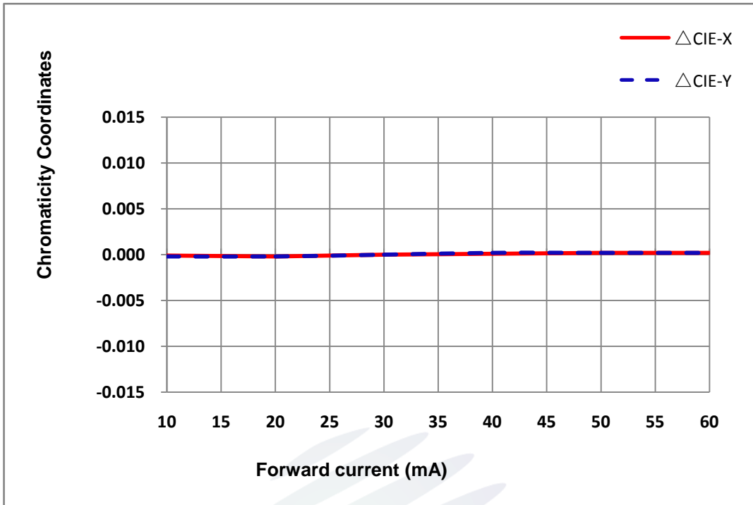
Fig. 1-13 Chromaticity Coordinate Shift Vs Forward Current 色坐标与电流特性曲线
