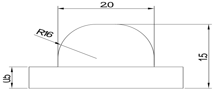
Fig.1-2 Side view 侧面视图
