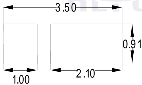
Fig.1-5 Soldering Patterns 推荐焊盘
