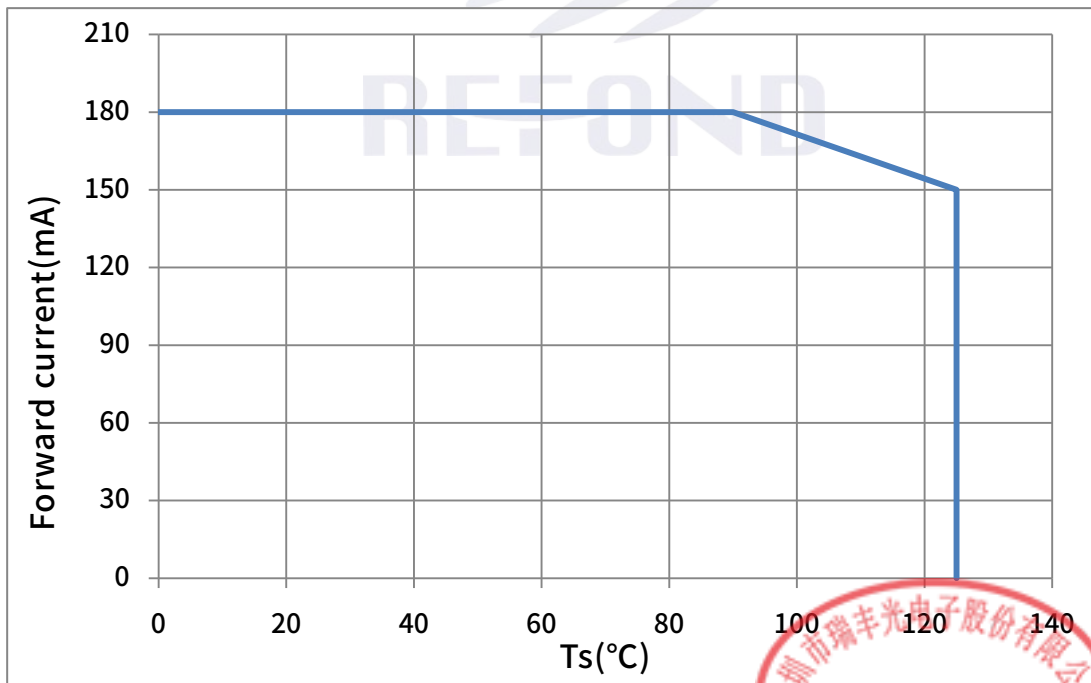
Fig. 1-10 Solder Temperature Vs Forward Current 管脚温度与正向电流特性曲线 Tj ≤ 150°C
