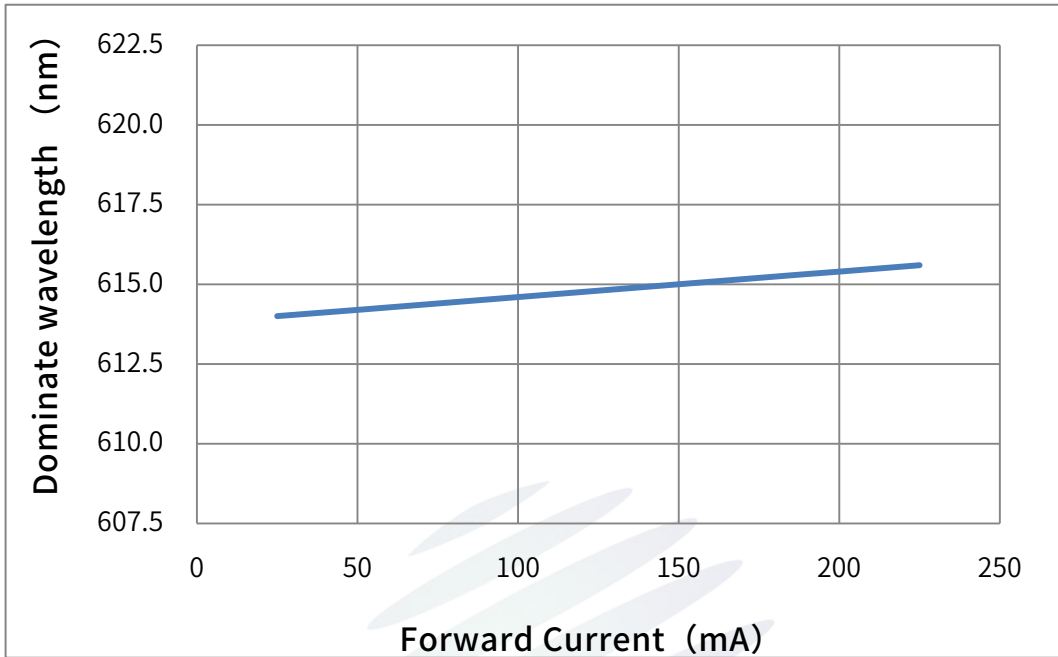
Fig. 1-12 Forward current vs. Dominate wavelength 正向电流与主波长特性曲线(Ts=25°C)
