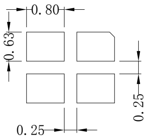
Fig.1-5 Soldering Patterns 推荐焊盘
