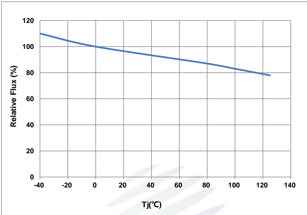
Fig. 1-9 Junction Temperature Vs Relative Flux结温与相对光强特性曲线
