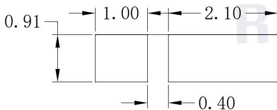
Fig.1-5 Soldering Patterns 推荐焊盘
