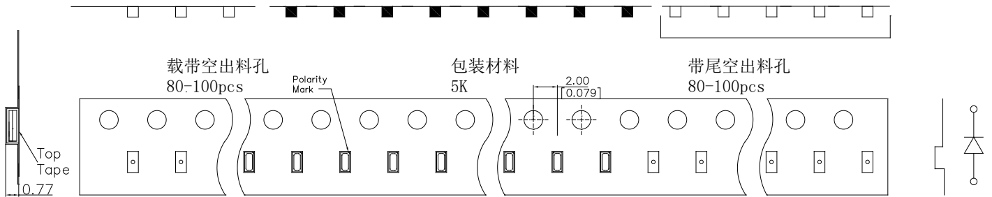
Fig.2-1 Carrier Tape Dimension 载带尺寸
