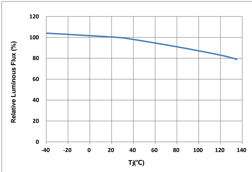
Fig. 1-9 Junction Temperature Vs Relative Intensity 结温与相对光通量特性曲线
