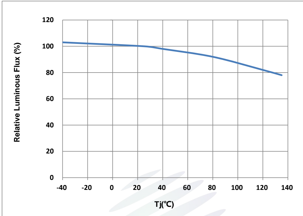
Fig. 1-9 Solder Temperature Vs Relative Intensity管脚温度与相对光通量特性曲线
