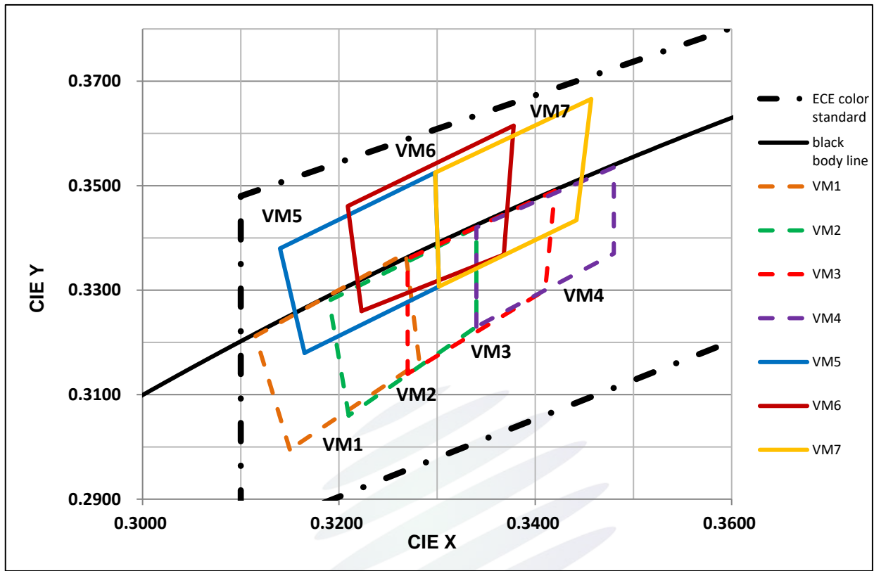
Fig. 1-6 The C.I.E Chromaticity Diagram CIE(White) CIE色度图 (白光)
